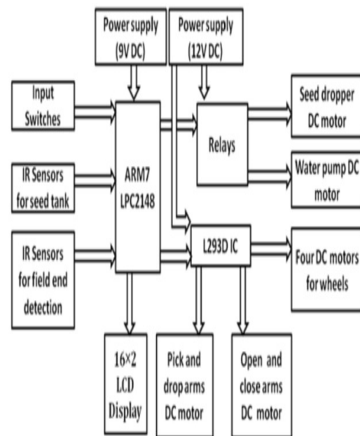
Fig 2. Block diagram
